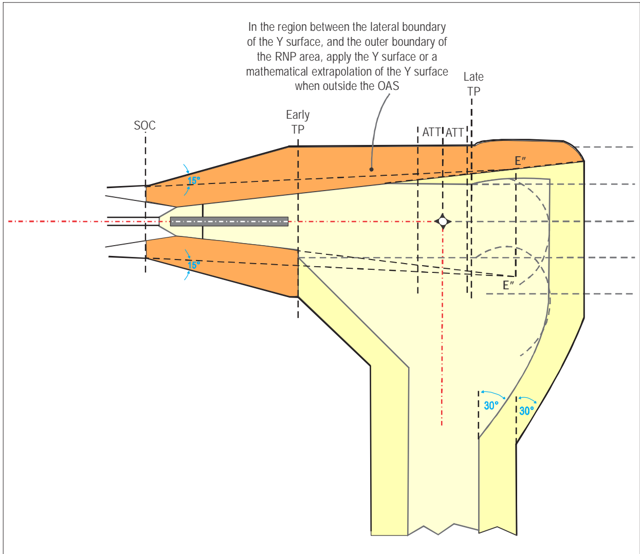
Figure II-1-3-23. Example: Transition to RNAV 1 or RNP 1, fly-by turn before the end of the precision segment
