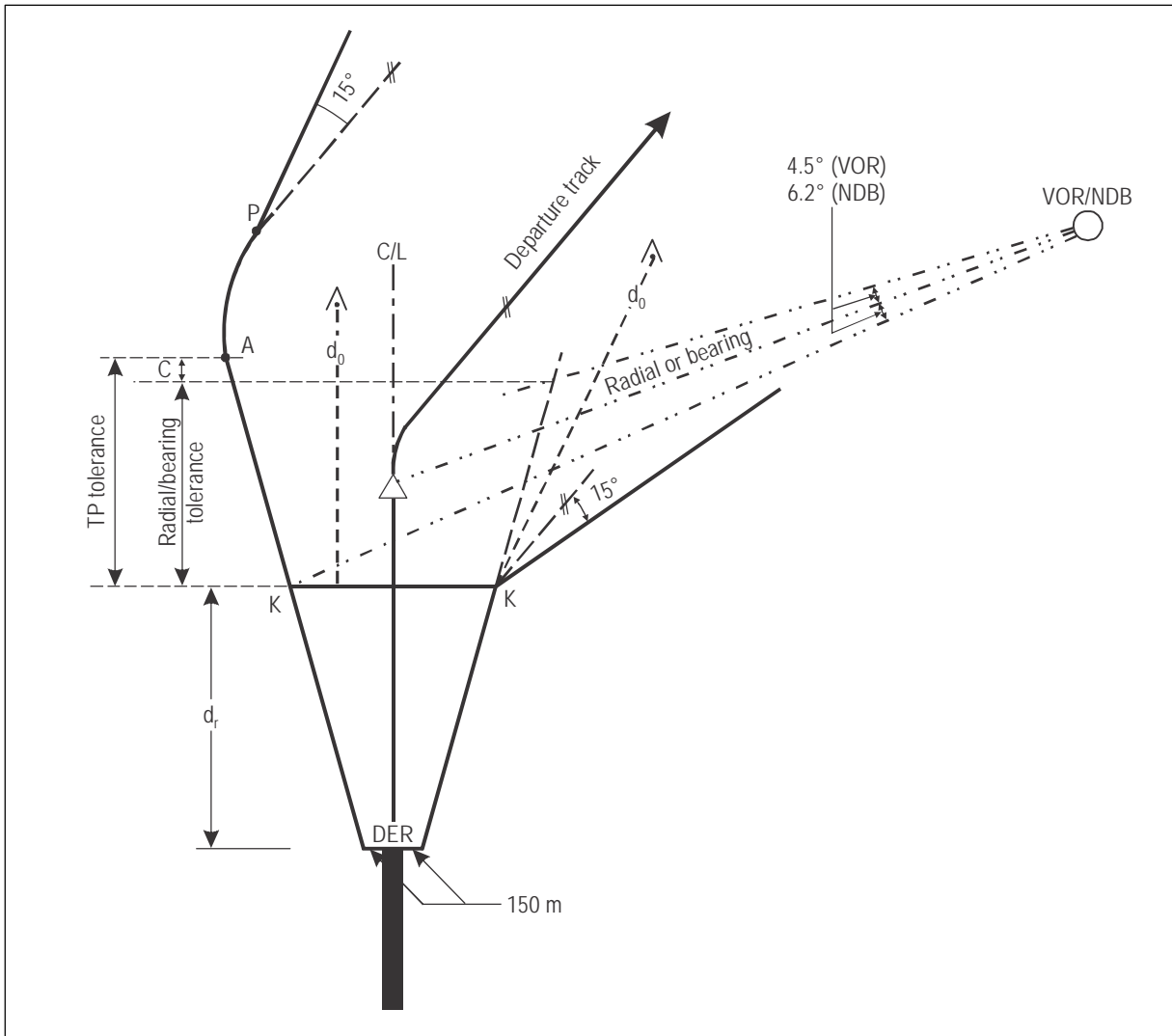
Figure I-3-3-11 a). Turning departure not overflying a facility — turning point tolerance area defined by intersecting radial
