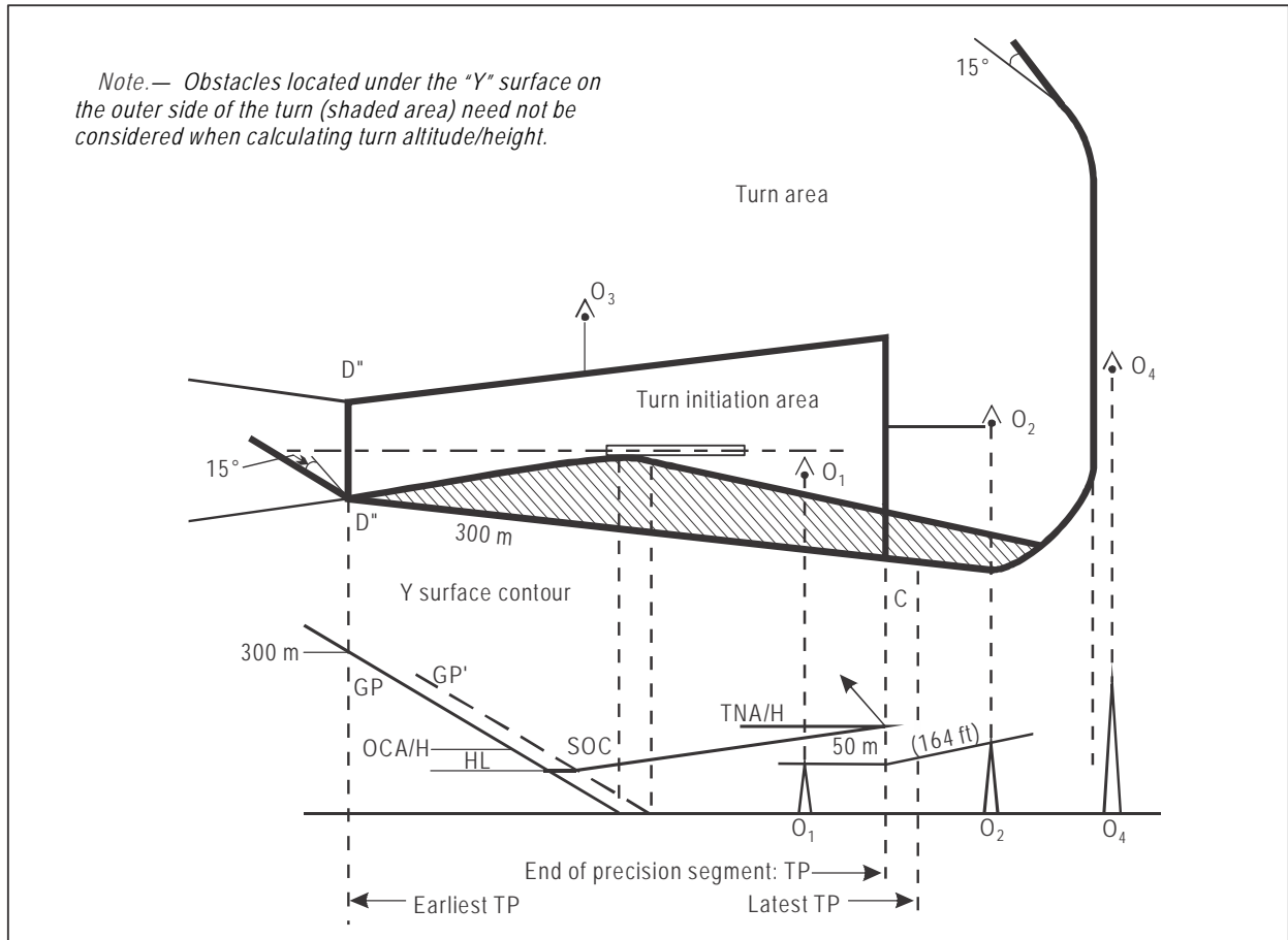
Figure II-1-3-20. Turn at a designated altitude
