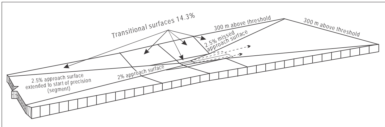
Figure II-1-3-9 b). Illustration of basic ILS surfaces as described in 3.4.7.2
