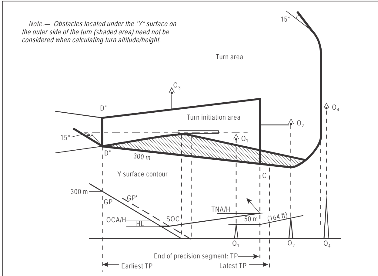
Figure III-3-6-18. Turn at a designated altitude
