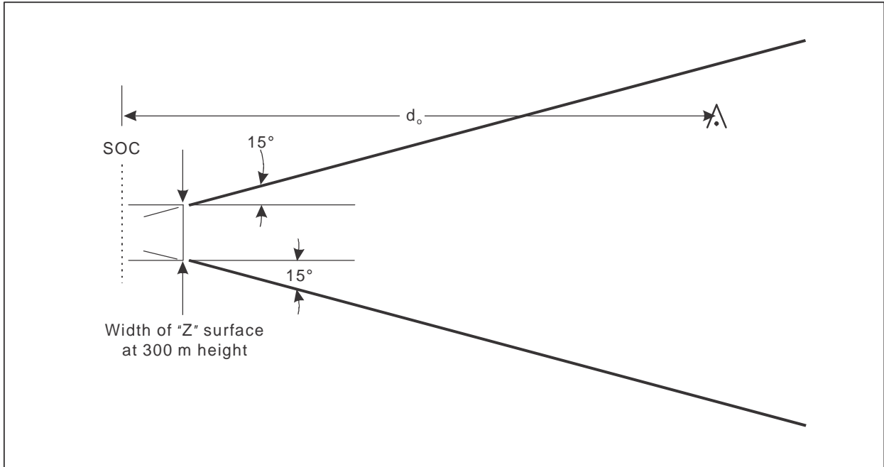
Figure II-1-1-17. Final segment of straight missed approach
