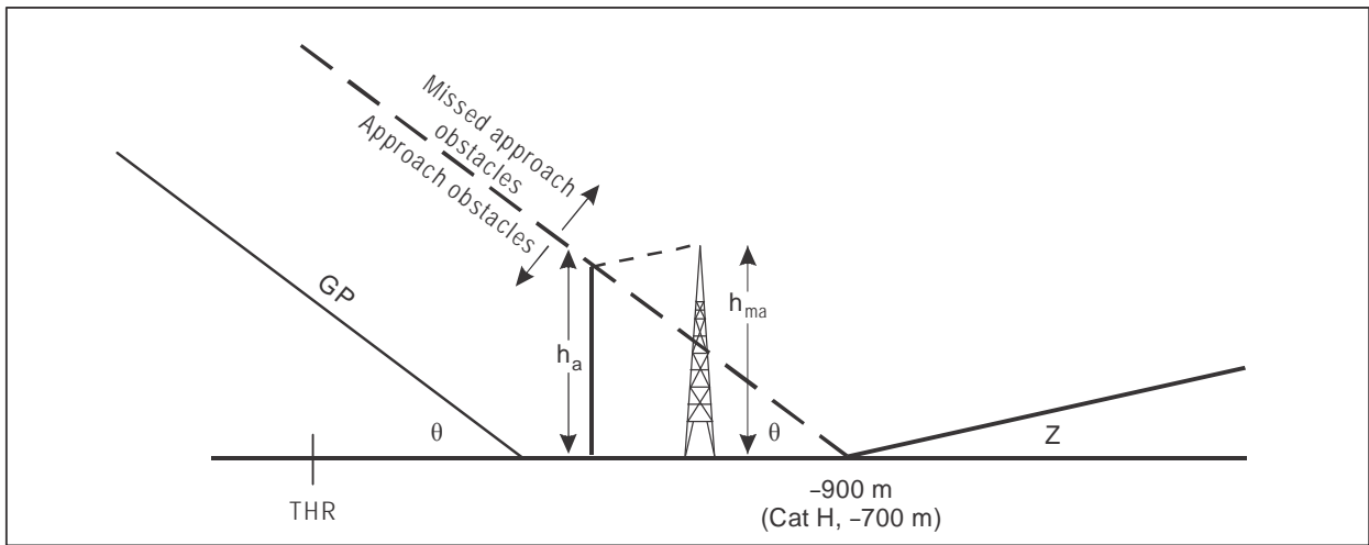
Figure II-1-1-16. Missed approach obstacle before range -900 m
