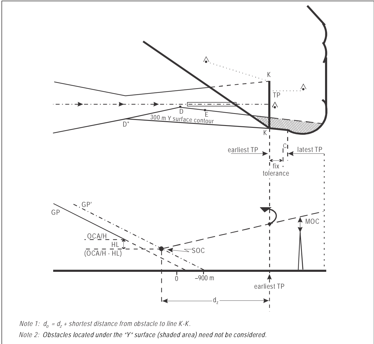
Figure II-1-3-21. Turn at designated TP (with TP fix)
