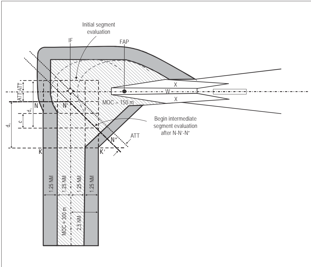
Figure III-3-6-5. Example: RNAV 1 or RNP 1 to GBAS transition, 90° intercept (max)
