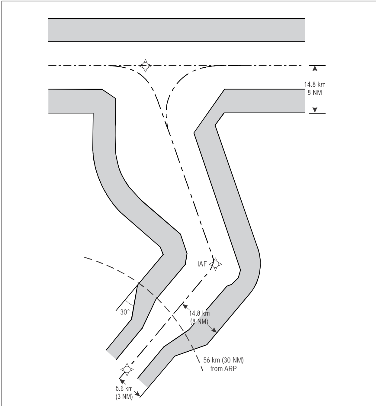
Figure I-4-2-5. GNSS arrival criteria, IAF beyond 56 km (30 NM) ARP: 14.8 km (8 NM) 1/2 AW prior to 56 km (30 NM) from ARP then 5.6 km (3 NM) 1/2 AW
