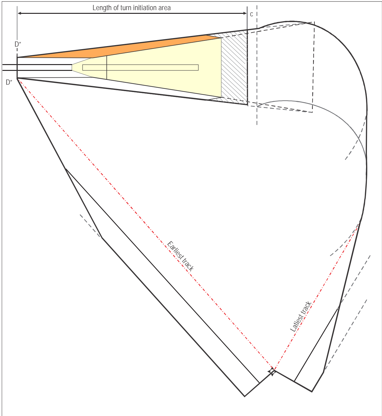
Figure III-3-6-23. Example: Turn at an altitude direct to an RNAV 1 or RNP 1 fix
