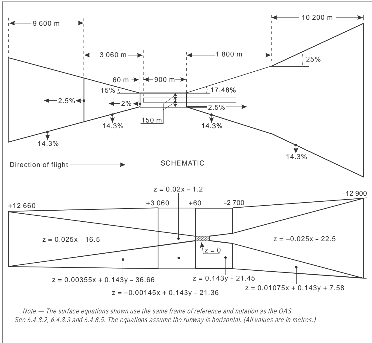
Figure III-3-6-8. Surface equations — basic ILS surfaces
