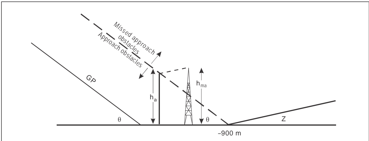
Figure II-1-3-17. Missed approach obstacle before range -900 m
