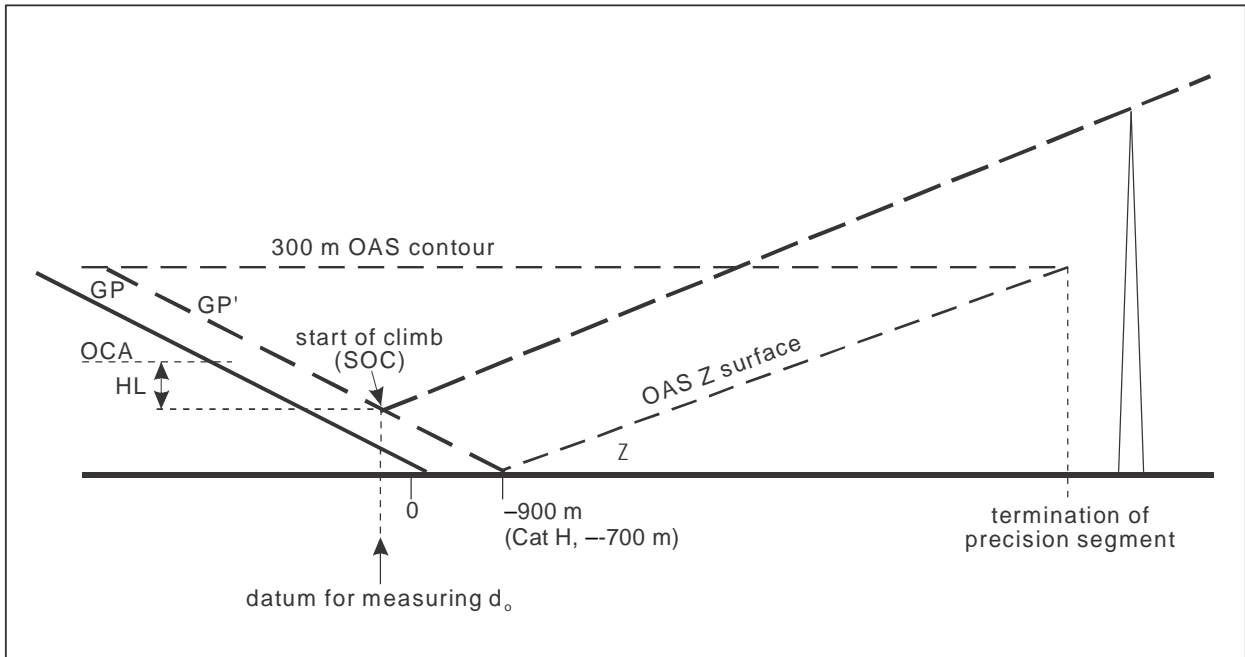
Figure II-1-1-18. Straight missed approach obstacle clearance
