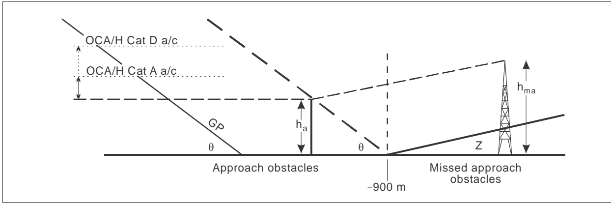
Figure II-1-3-16. Missed approach obstacle after range -900 m
