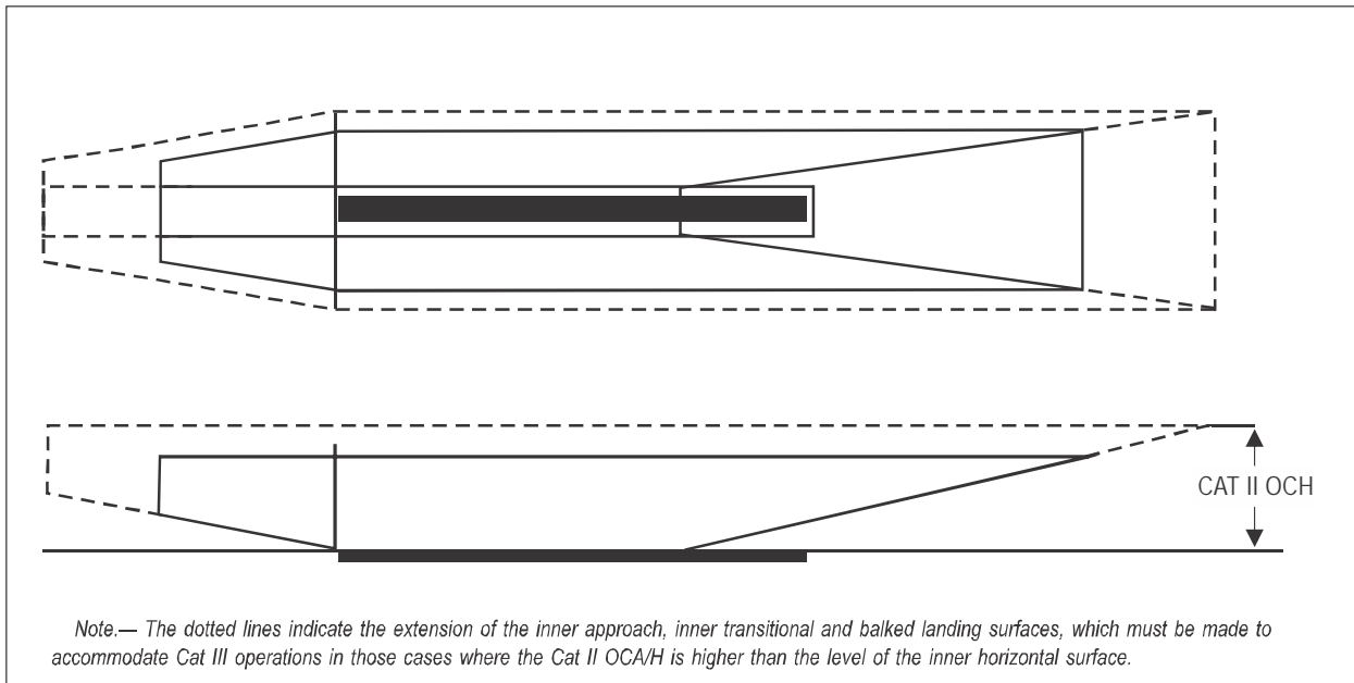
Figure II-1-1-8 b). Illustration of basic ILS surfaces as described in 1.4.7.2
