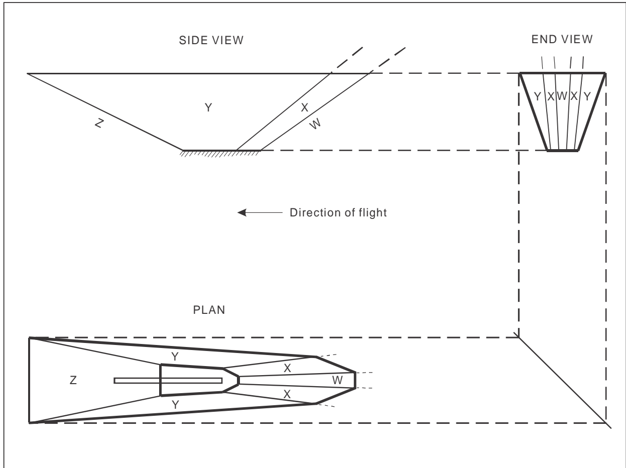
Figure II-1-3-11. Illustrations of ILS obstacle assessment surfaces
