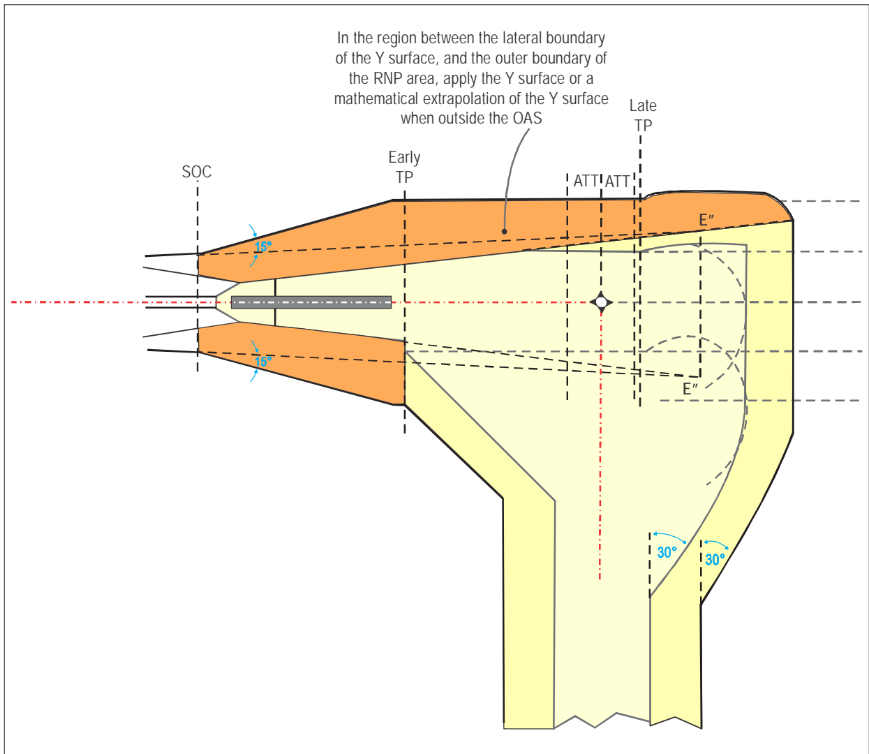
Figure III-3-6-22. Example: Transition to RNAV 1 or RNP 1, fly-by turn before the end of the precision segment
