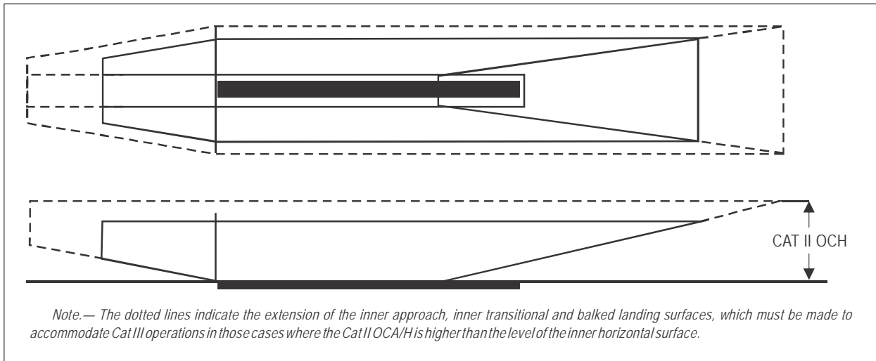
Figure II-1-3-9 a). Annex 14 inner approach, inner transitional and balked landing surfaces as applied for obstacle assessment for Cat II and III ILS operations
