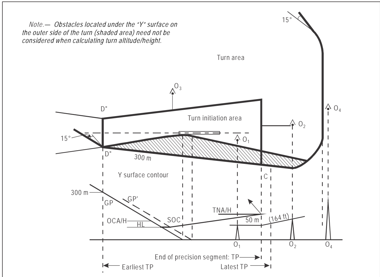
Figure II-1-1-19. Turn at a designated altitude
