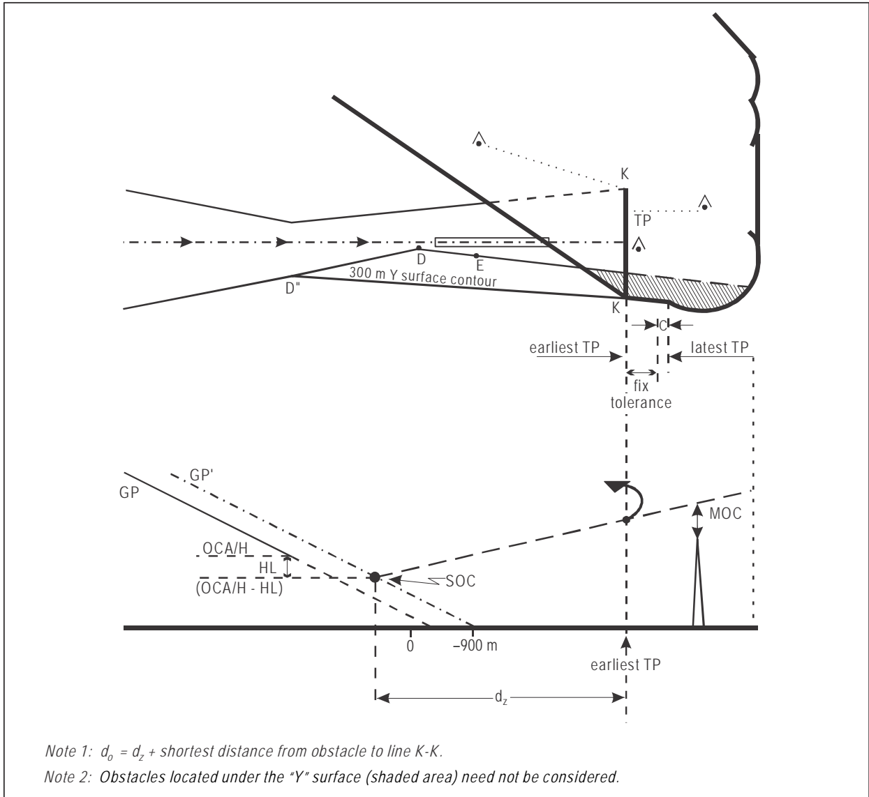
Figure III-3-6-19. Turn at designated TP (with TP fix)
