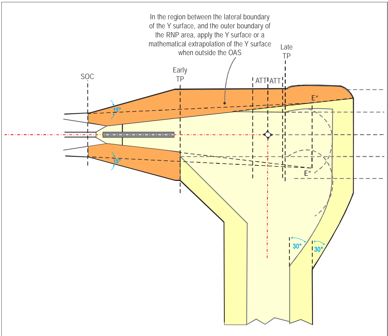
Figure II-1-1-22. Example: Transition to RNAV 1 or RNP 1, fly-by turn before the end of the precision segment
