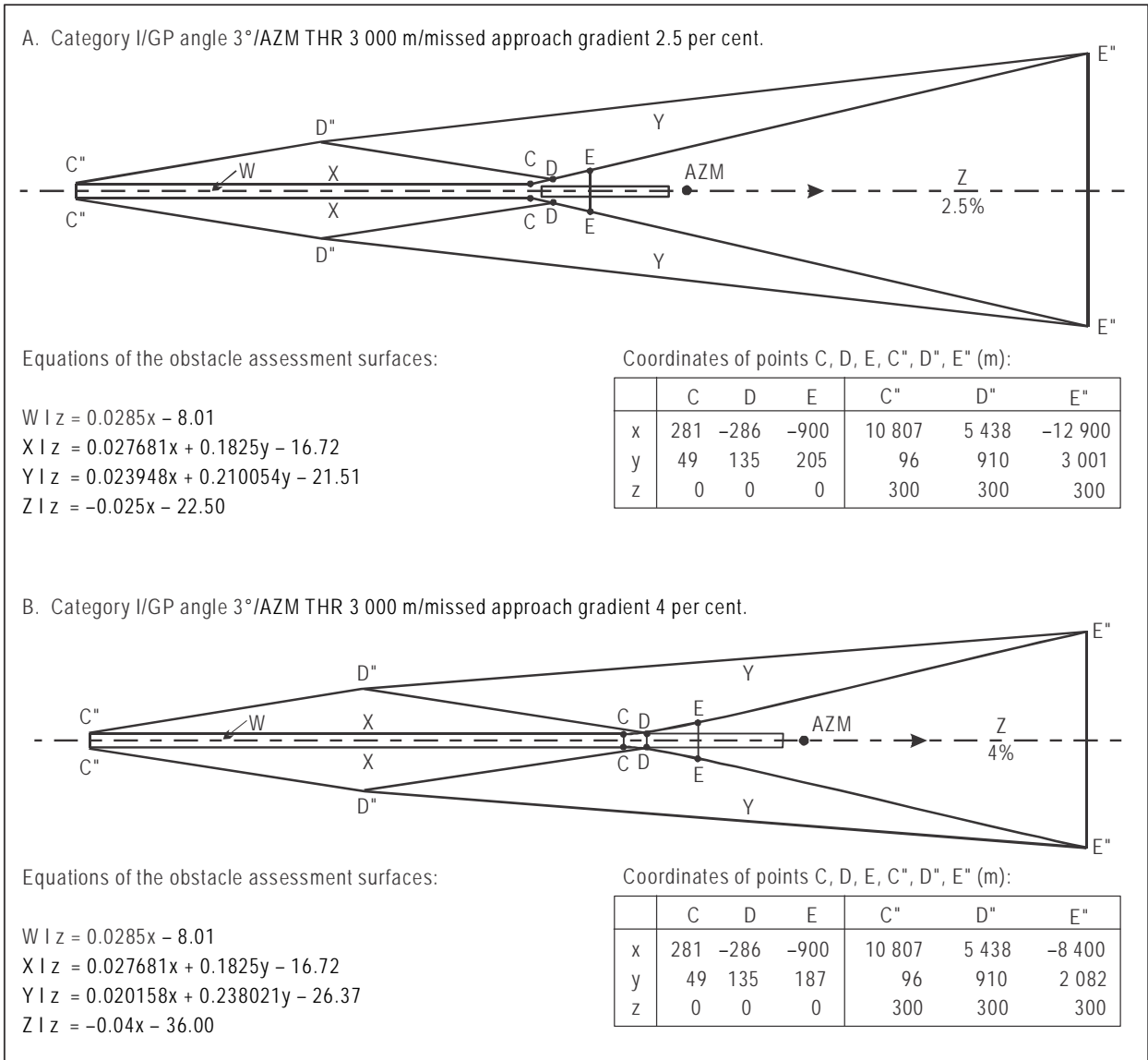
Figure III-3-6-12. Typical OAS contours for standard size aircraft
