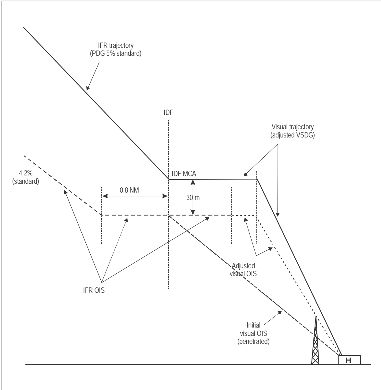
Figure IV-1.3. Mitigation of OIS penetration by raising the VSDG
