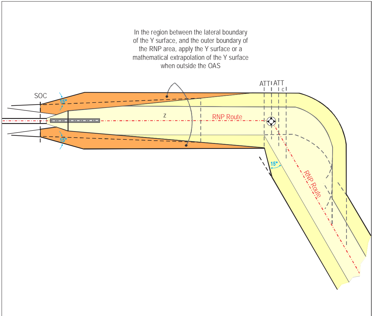
Figure II-1-3-22. Example: Transition to RNP 1, flyover turn after the precision segment
