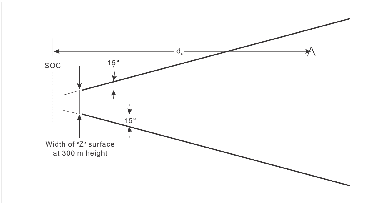
Figure III-3-6-16. Final segment of straight missed approach
