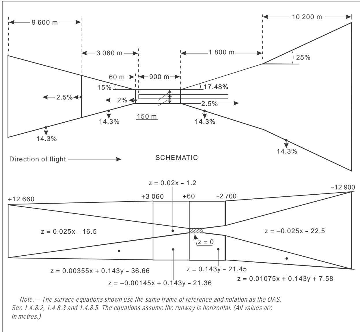
Figure II-1-1-9. Surface equations — basic ILS surfaces
