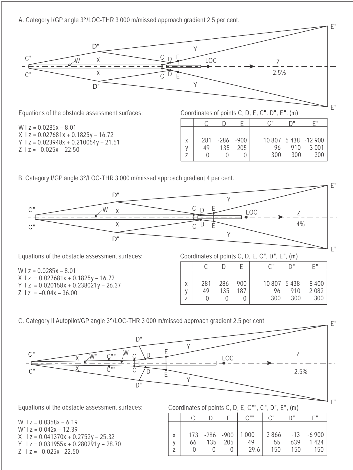
Figure II-1-13. Typical OAS contours for standard size aircraft
