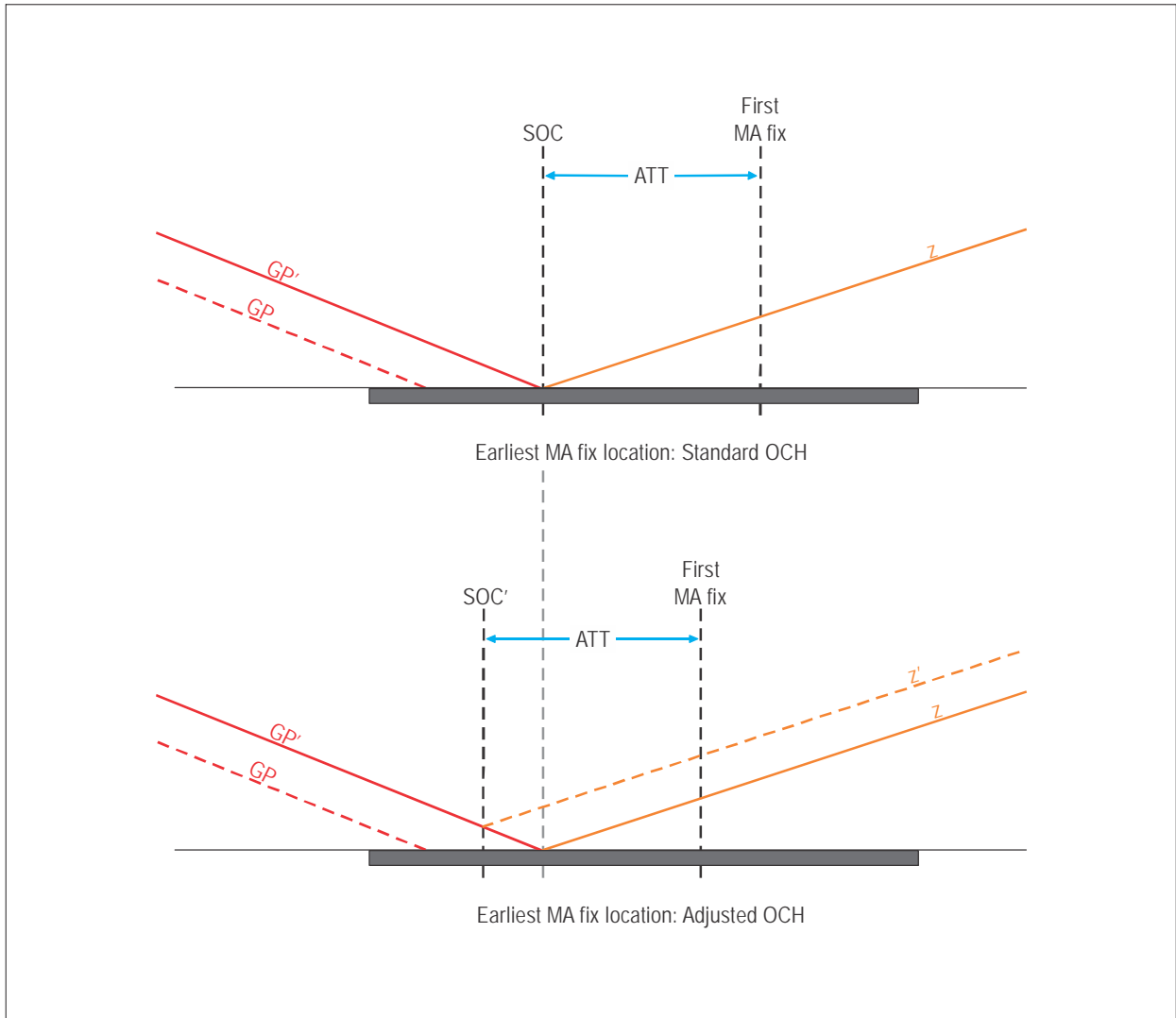
Figure II-1-3-25. Earliest fix location for RNAV or RNP missed approach
