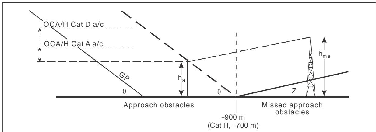
Figure III-3-6-14. Missed approach obstacle after range -900 m
