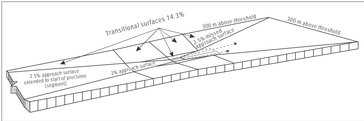
Figure III-3-6-7. Illustration of basic ILS surfaces as described in Part III, Section 3, Chapter 6, 6.4.7.2
