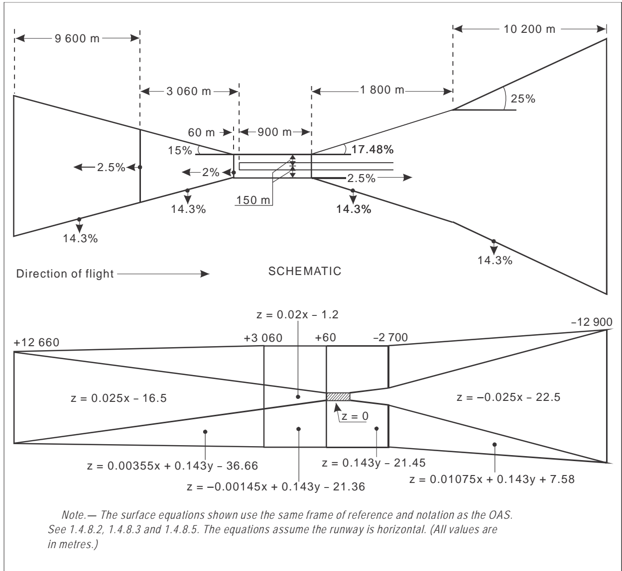
Figure II-1-3-10. Surface equations — basic ILS surfaces
