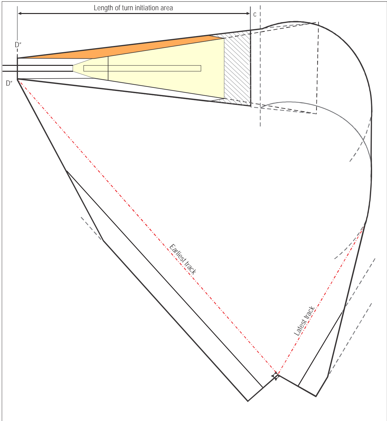
Figure II-1-1-23. Example: Turn at an altitude direct to an RNAV 1 or RNP 1 fix
