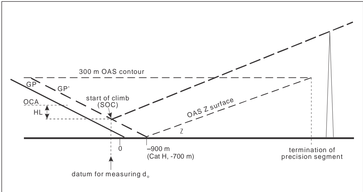
Figure III-3-6-17. Straight missed approach obstacle clearance
