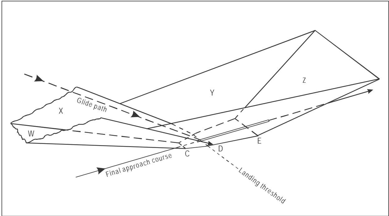
Figure III-3-6-10. Illustration of ILS obstacle assessment surfaces for GBAS operations — perspective view
