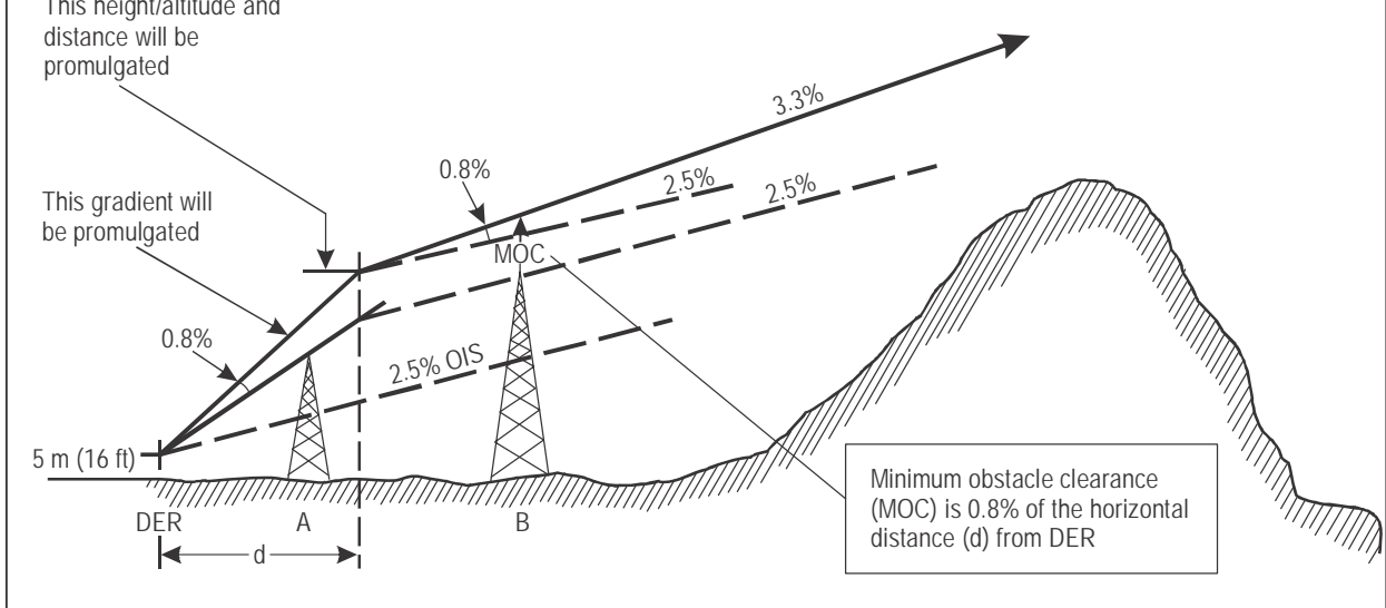
Figure I-3-5-1. Climb gradient reduction in departure
