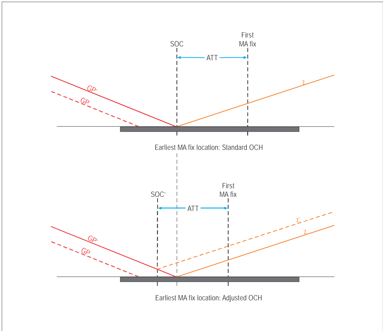
Figure II-1-1-24. Example: Earliest fix location for RNAV or RNP missed approach
