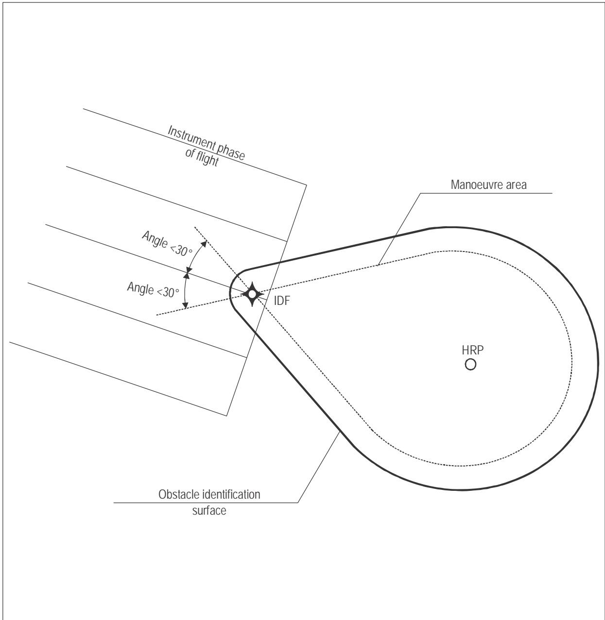
Figure IV-1-8. Manoeuvring visual segment representation of the level OIS if the initial take-off can be performed in an omni-directional way
