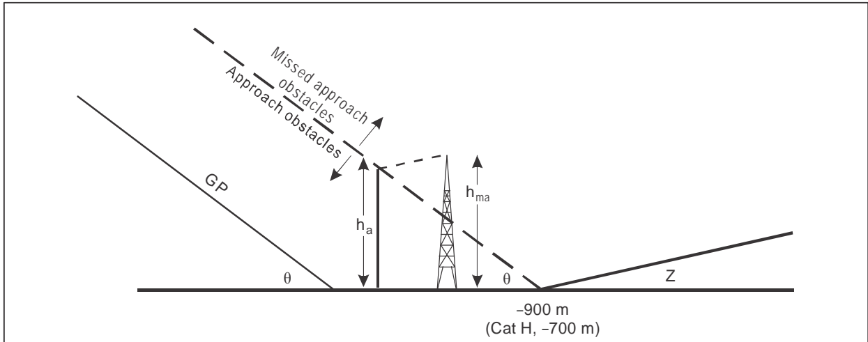
Figure III-3-6-15. Missed approach obstacle before range -900 m
