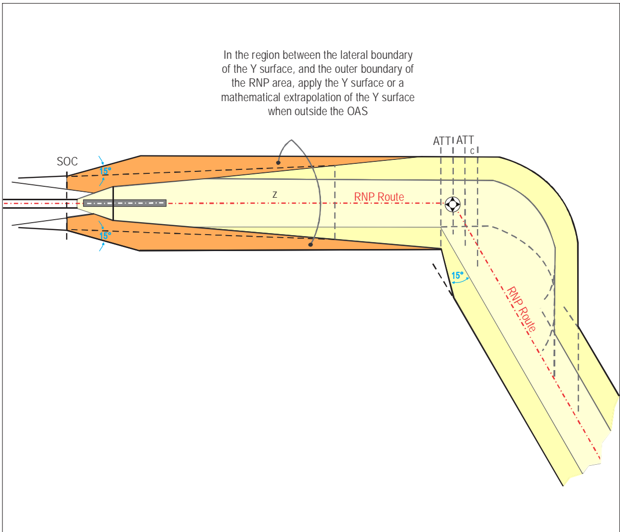
Figure II-1-1-21. Example: Transition to RNP 1, flyover turn after the precision segment
