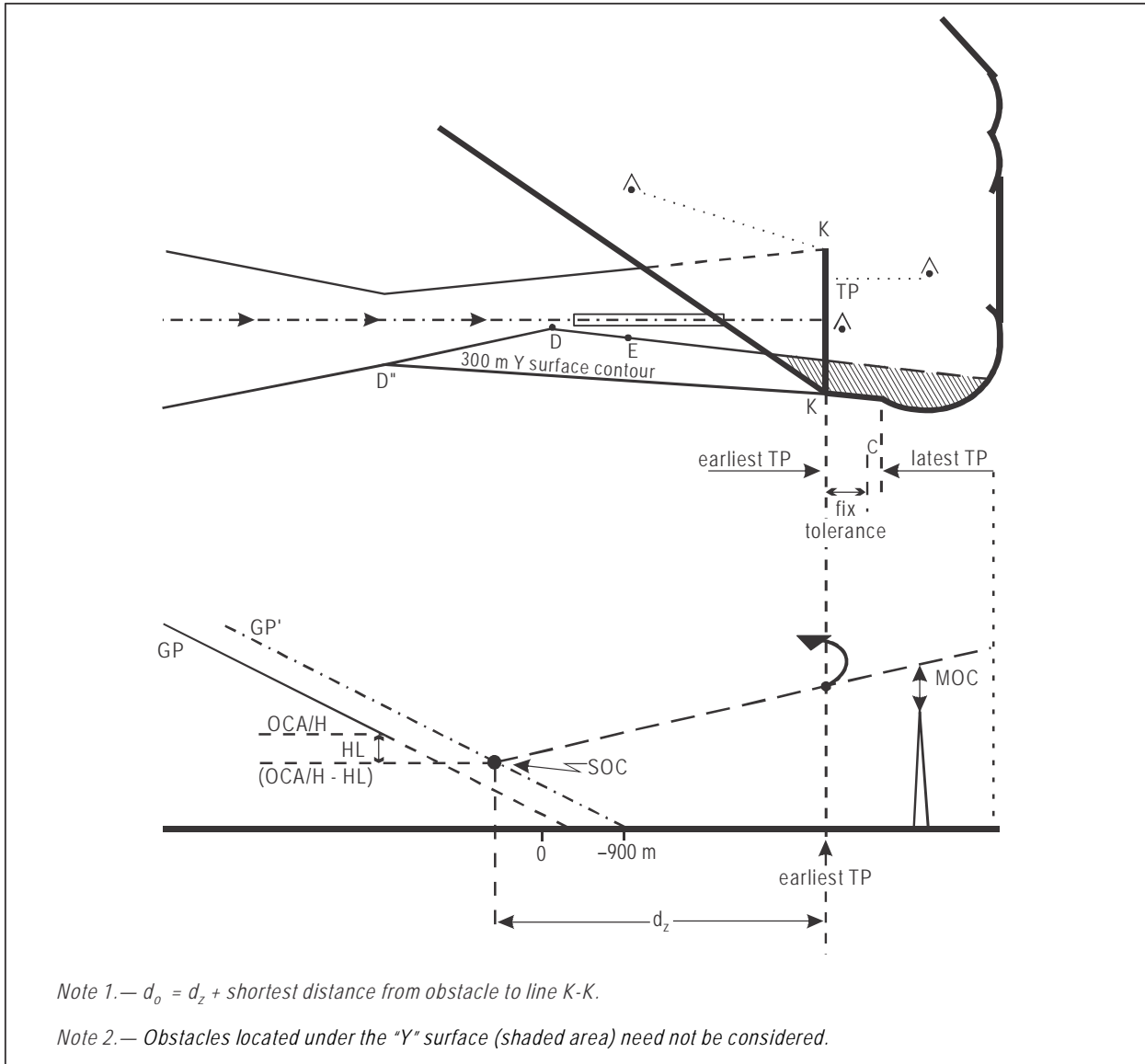
Figure II-1-1-20. Turn at designated TP (with TP fix)
