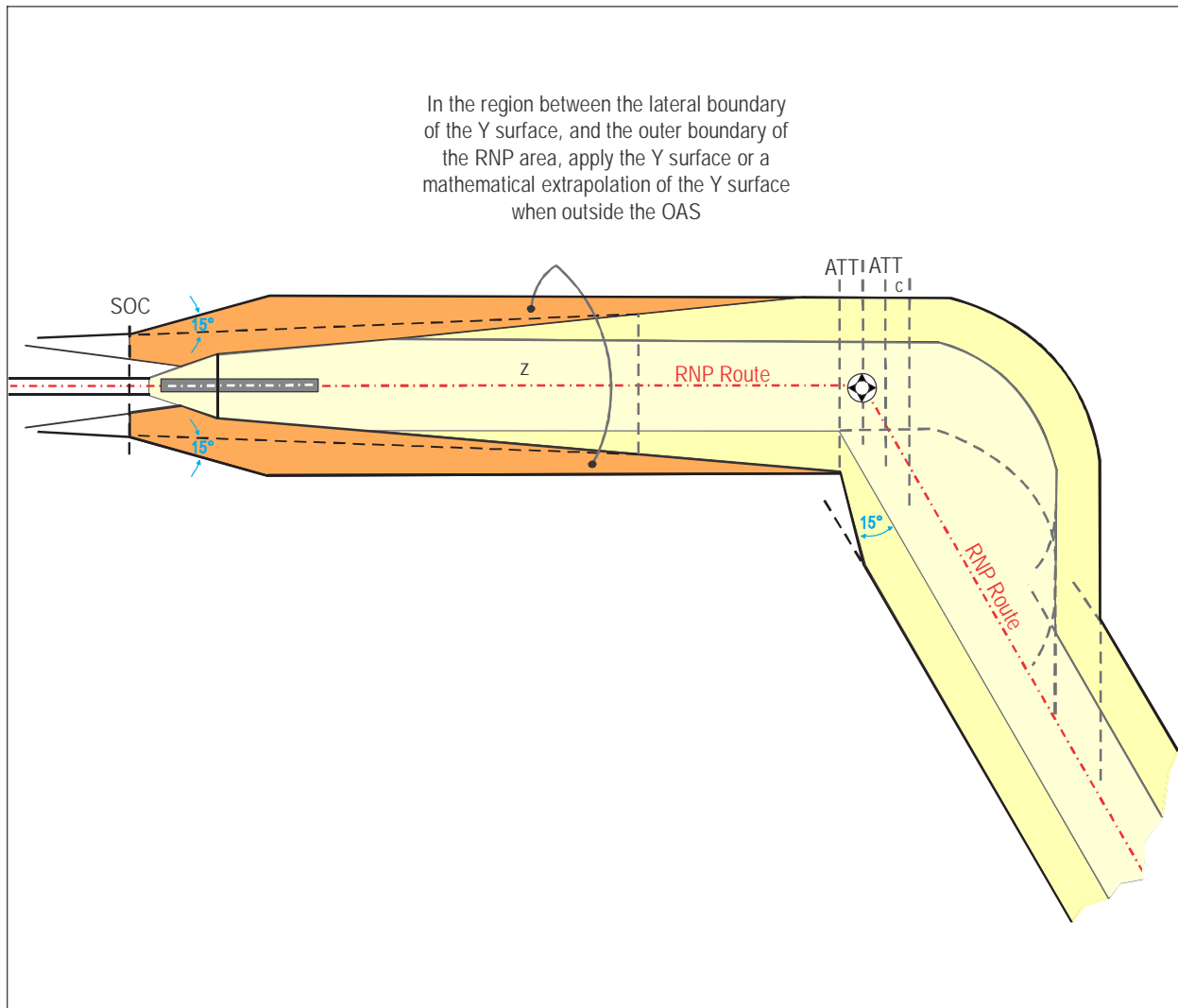
Figure III-3-6-21. Example: Transition to RNP 1, flyover turn after the precision segment
