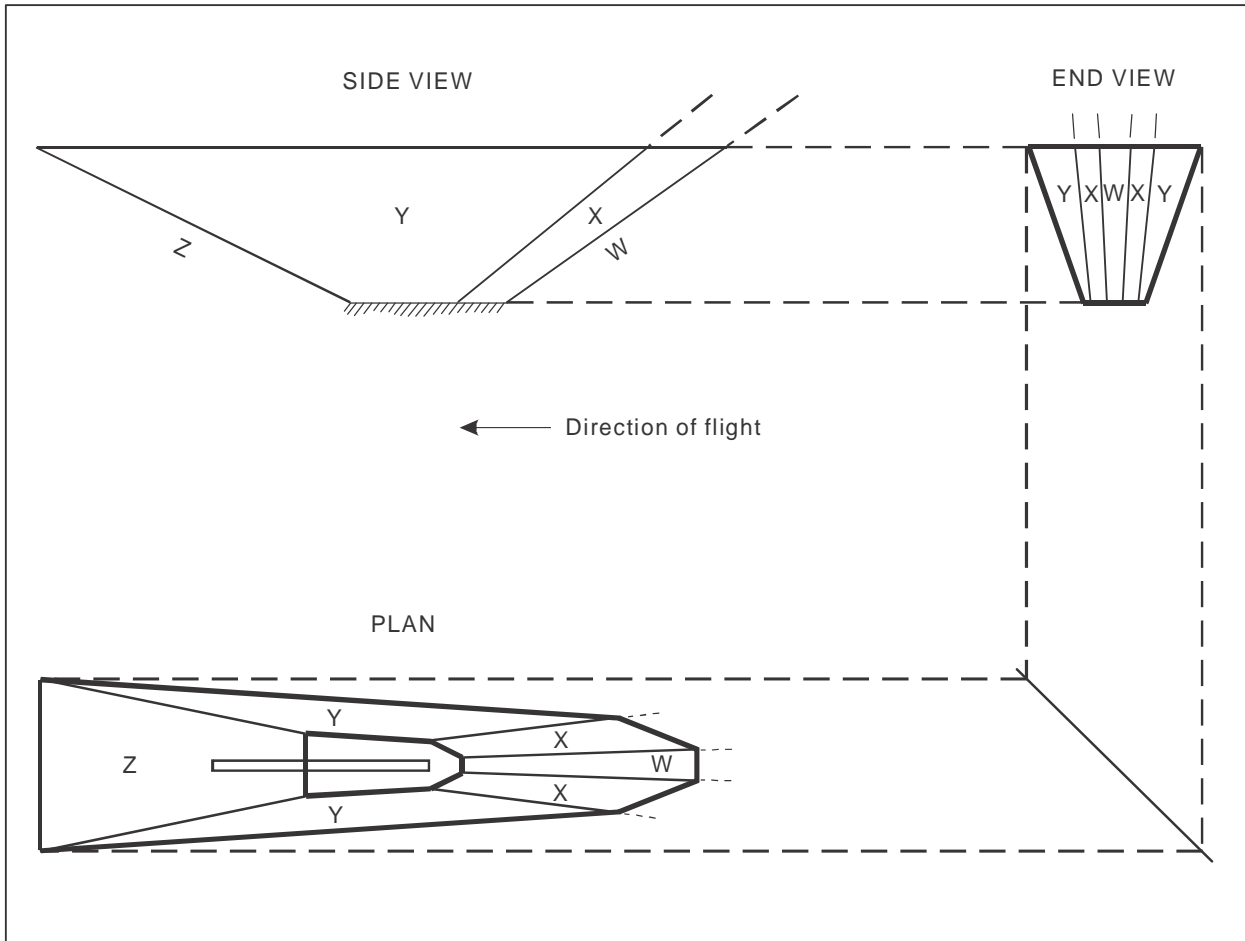
Figure II-1-1-10. Illustrations of ILS obstacle assessment surfaces
