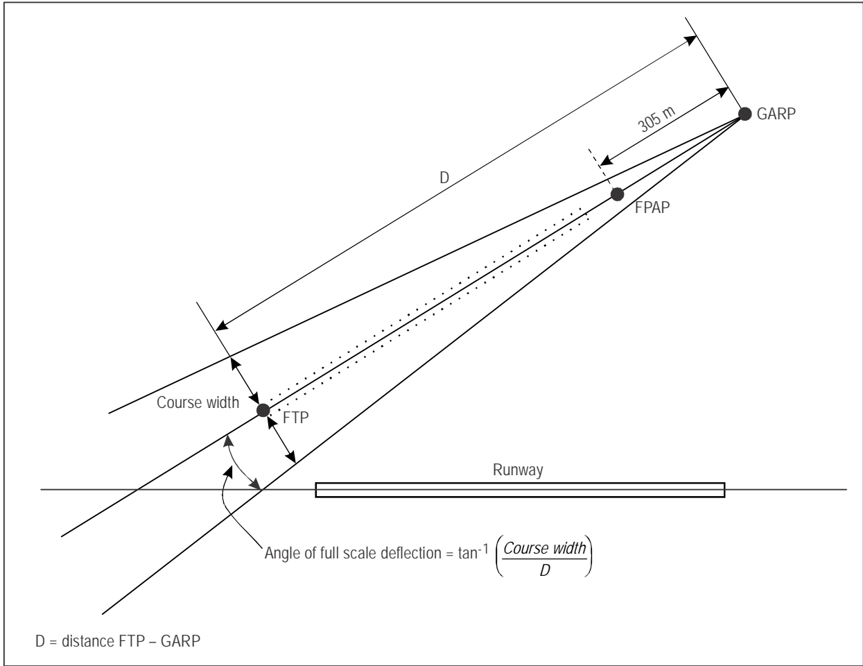
Figure III-3-6-20. GBAS Cat I with offset azimuth final approach course alignment
