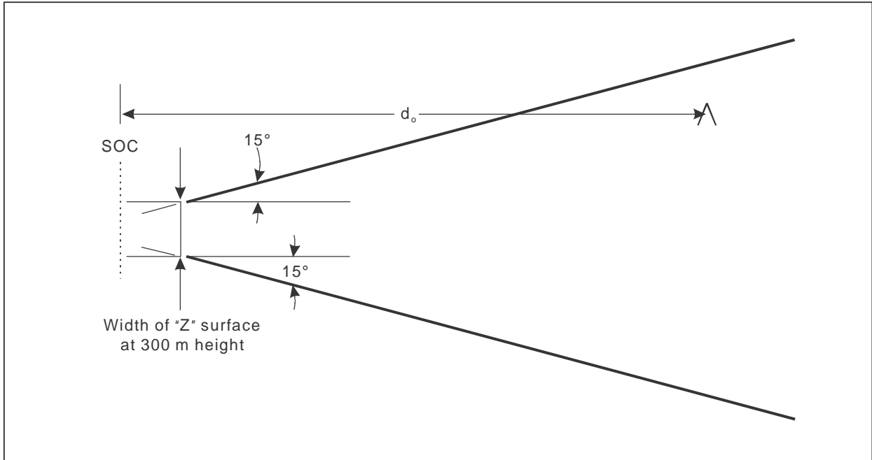
Figure II-1-3-18. Final segment of straight missed approach
