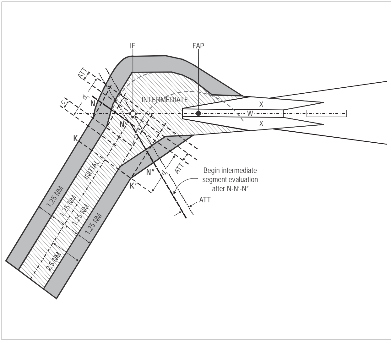
Figure III-3-6-4. Example: RNAV 1 or RNP 1 to GBAS transition, 60° intercept
