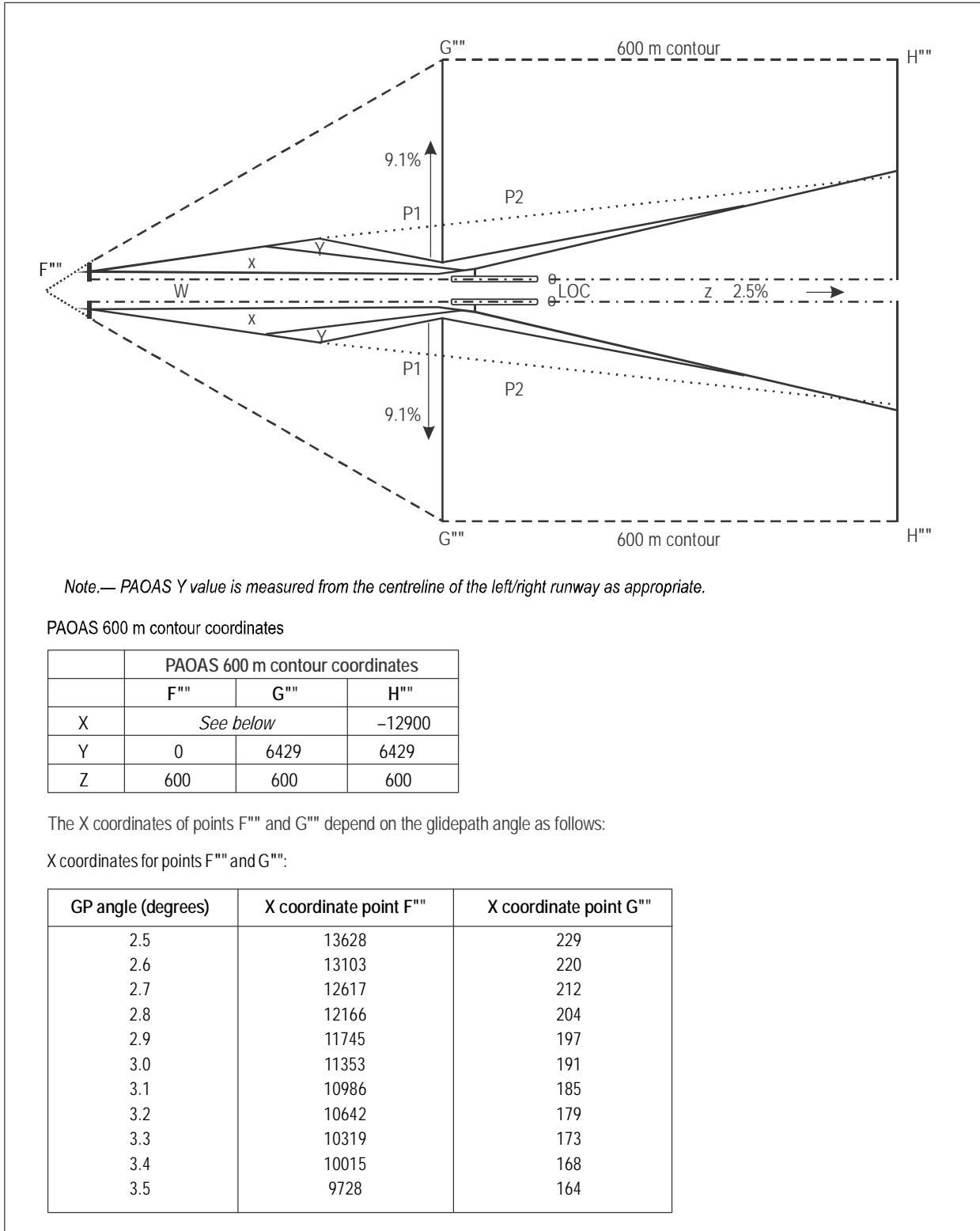
Figure II-1-1-App D-1. Example of PAOAS and OAS contours
