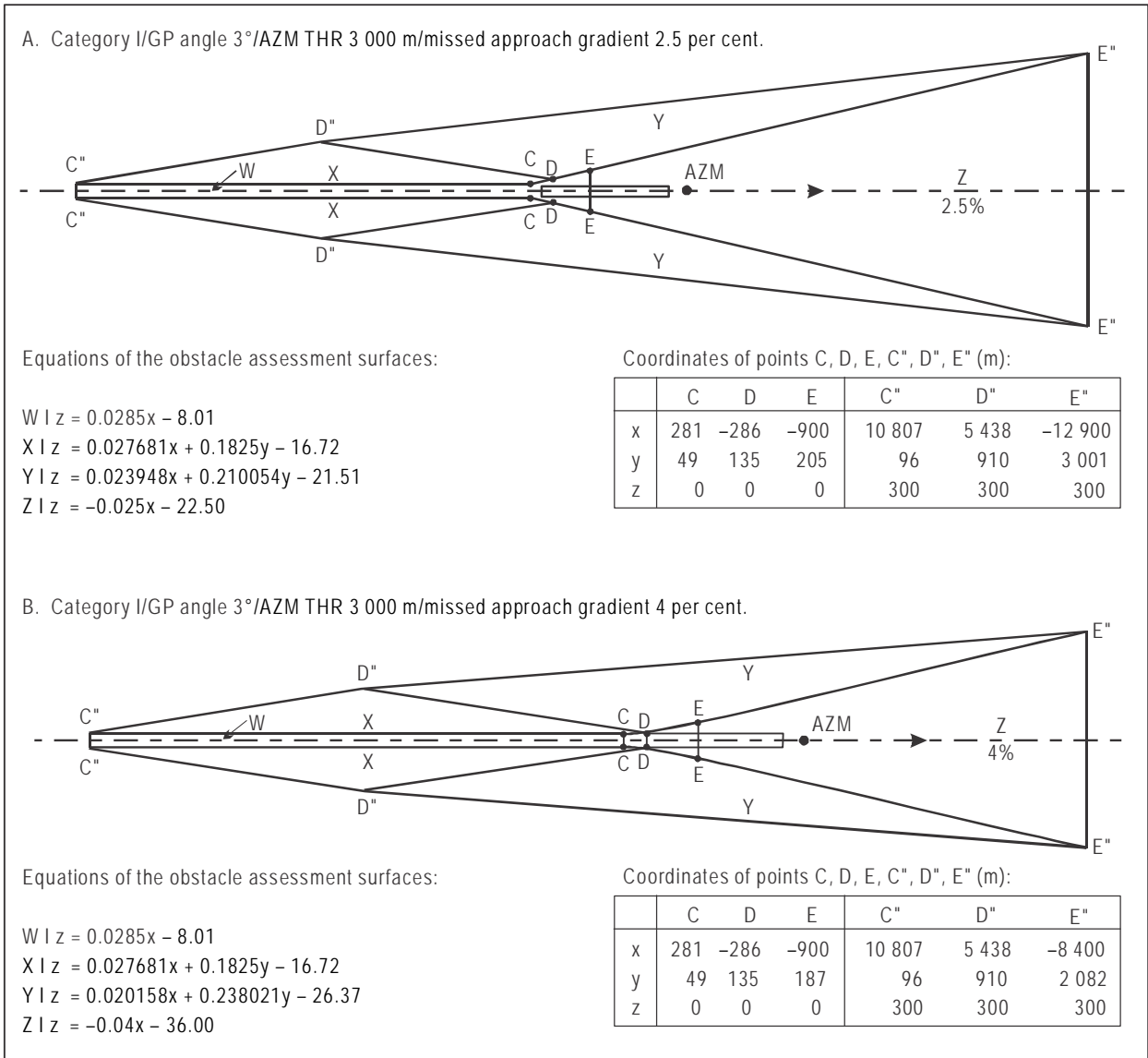
Figure II-1-3-14. Typical OAS contours for standard size aircraft
