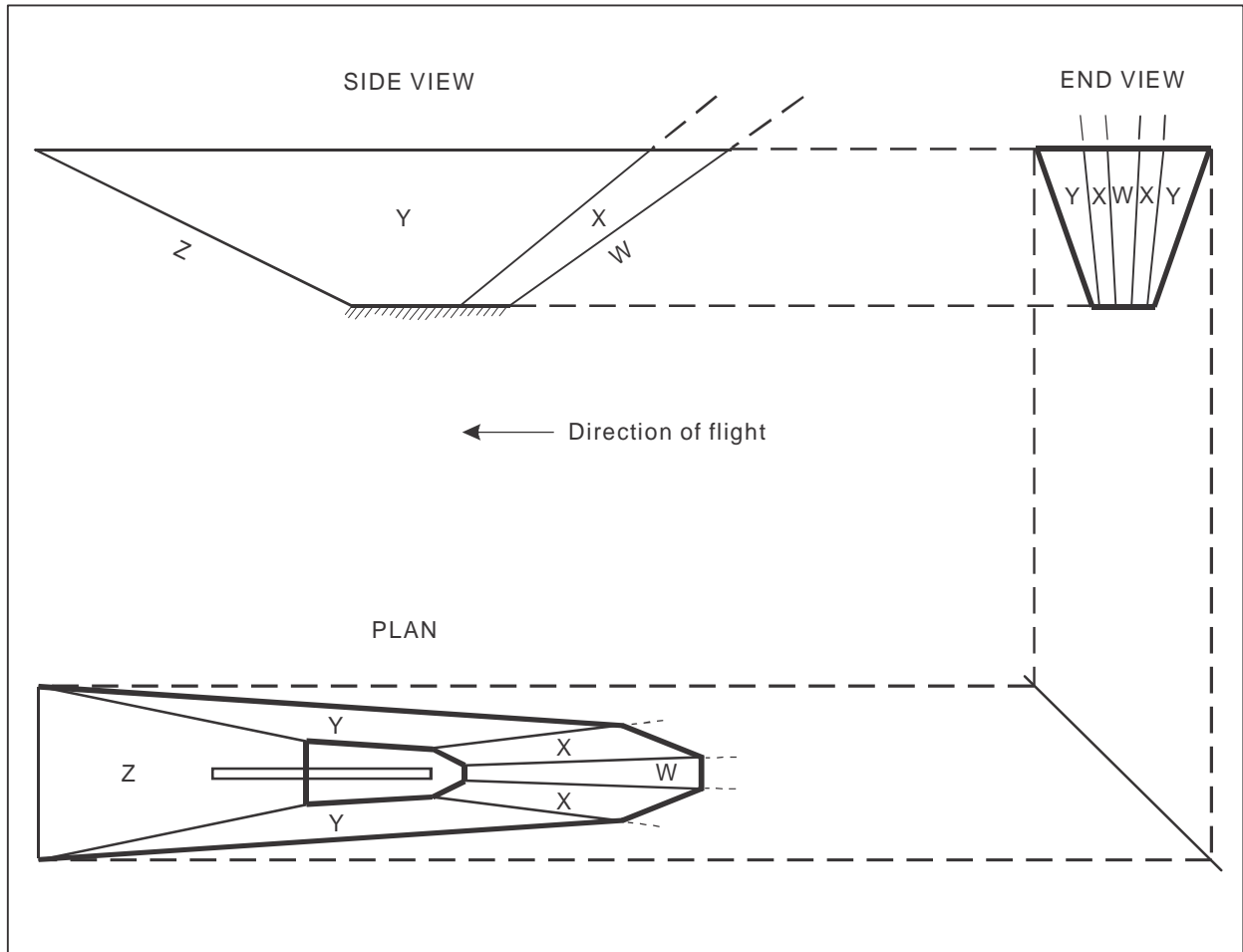
Figure III-3-6-9. Illustration of ILS obstacle assessment surfaces for GBAS operations
