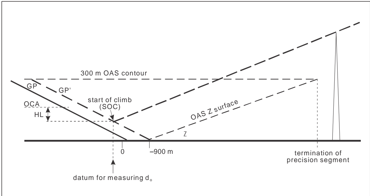
Figure II-1-3-19. Straight missed approach obstacle clearance
