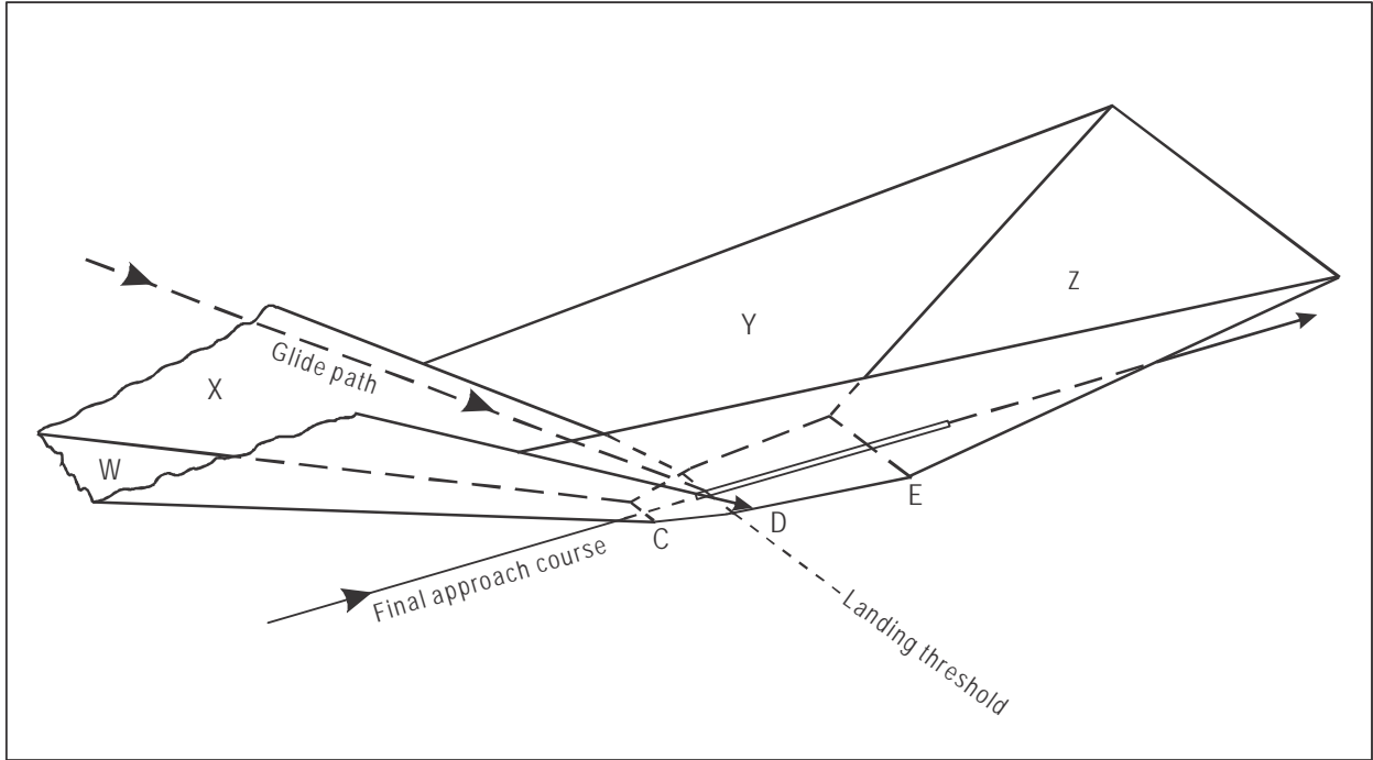
Figure II-1-1-11. Illustrations of ILS obstacle assessment surfaces — perspective view
