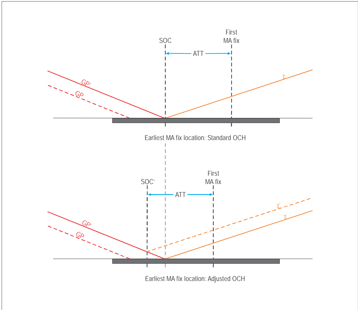
Figure III-3-6-24. Earliest fix location for RNAV or RNP missed approach
