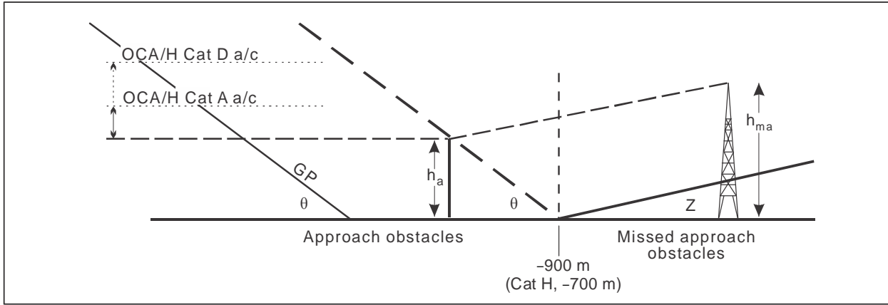
Figure II-1-1-15. Missed approach obstacle after range -900 m
