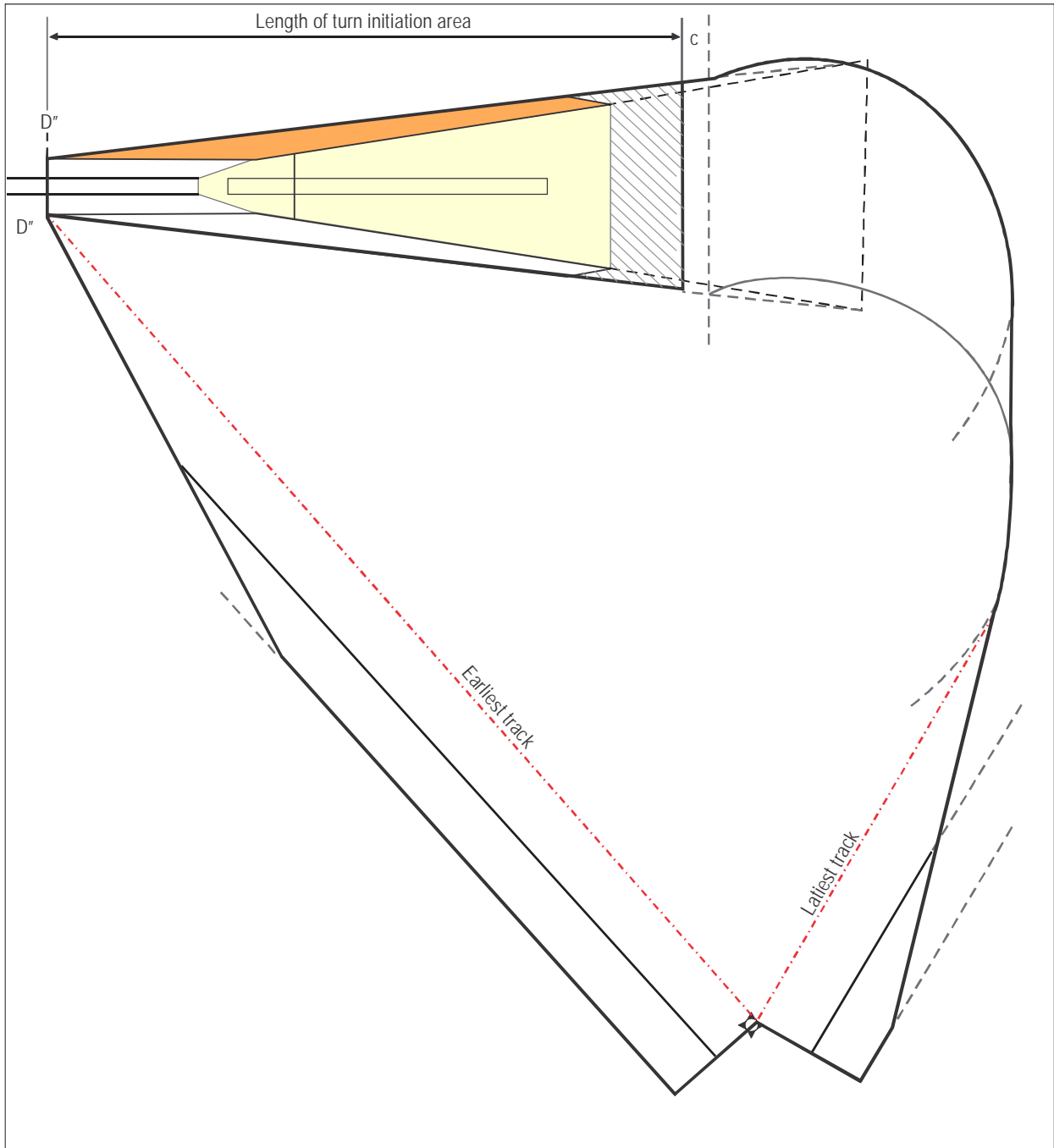
Figure II-1-3-24. Example: Turn at an altitude direct to an RNAV 1 or RNP 1 fix
