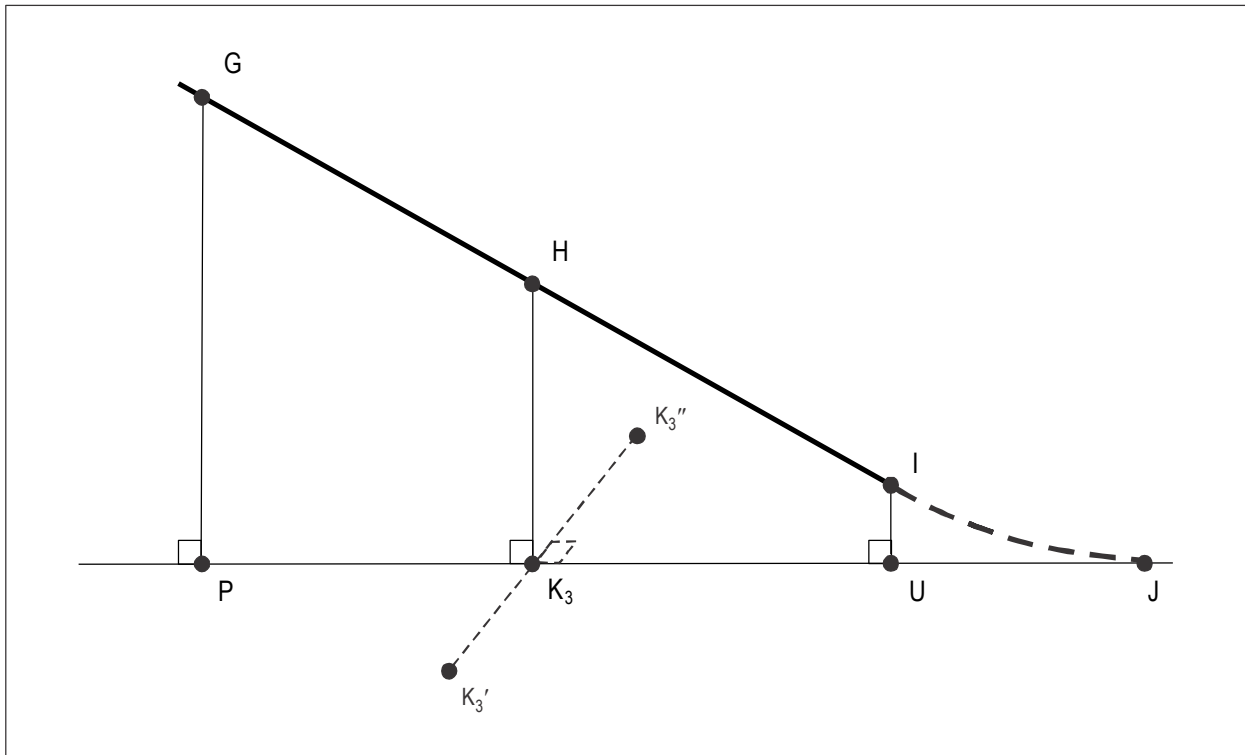
Figure A2-9. Reference helicopter approach profile characteristics
