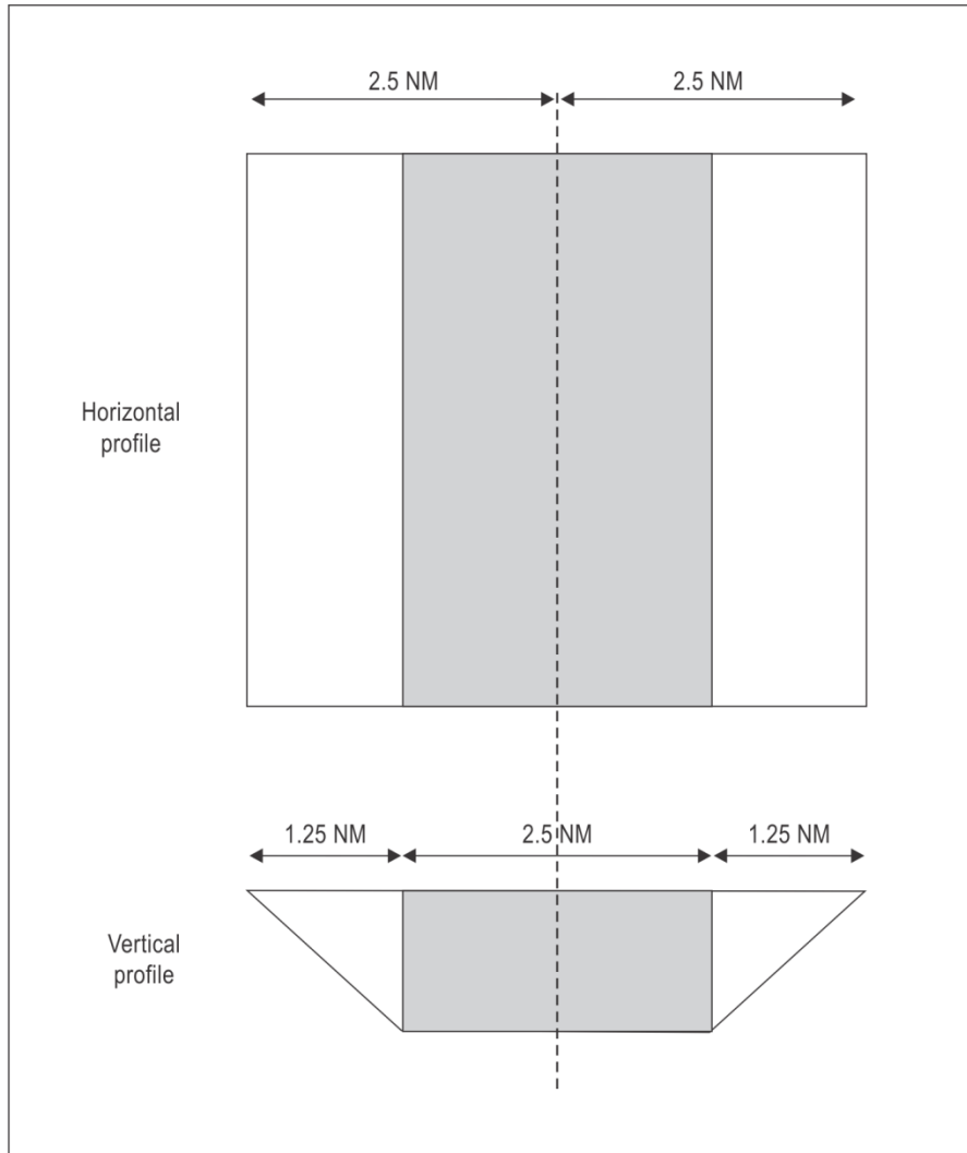
Figure A-2-5. Area width for an RNP 1 STAR between 15 NM and 30 NM from the ARP
