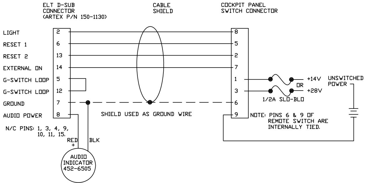
Figure 12 – Wiring Diagram: Composite Airframe
