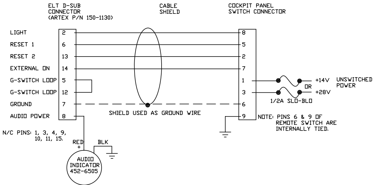
Figure 10 – Wiring Diagram: Metal Airframe
