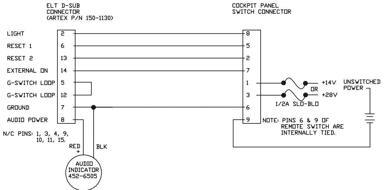
Figure 13 – Wiring Diagram: Composite Airframe
