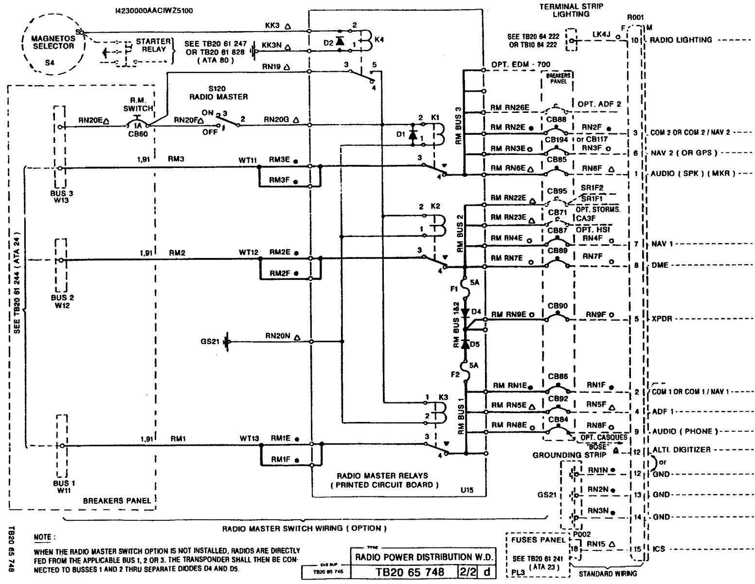
Figure 11.6.23.10.8C (2 / 2) - DISTRIBUTION RADIO - RADIO POWER DISTRIBUTION OPT10 J894 00M/10M/20M/30M
