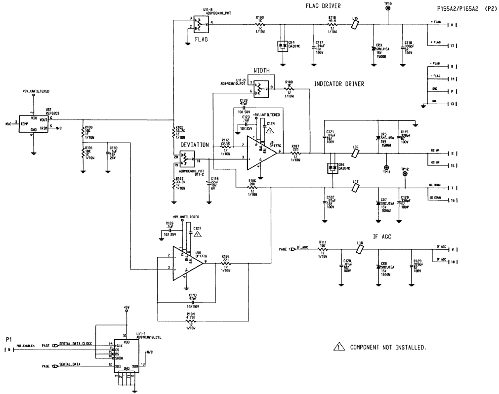
Figure 6-29 Gilleslope Board Schematic (Dwg No. 002-09060-0000 rev. D, Sheet 3 of 3)
